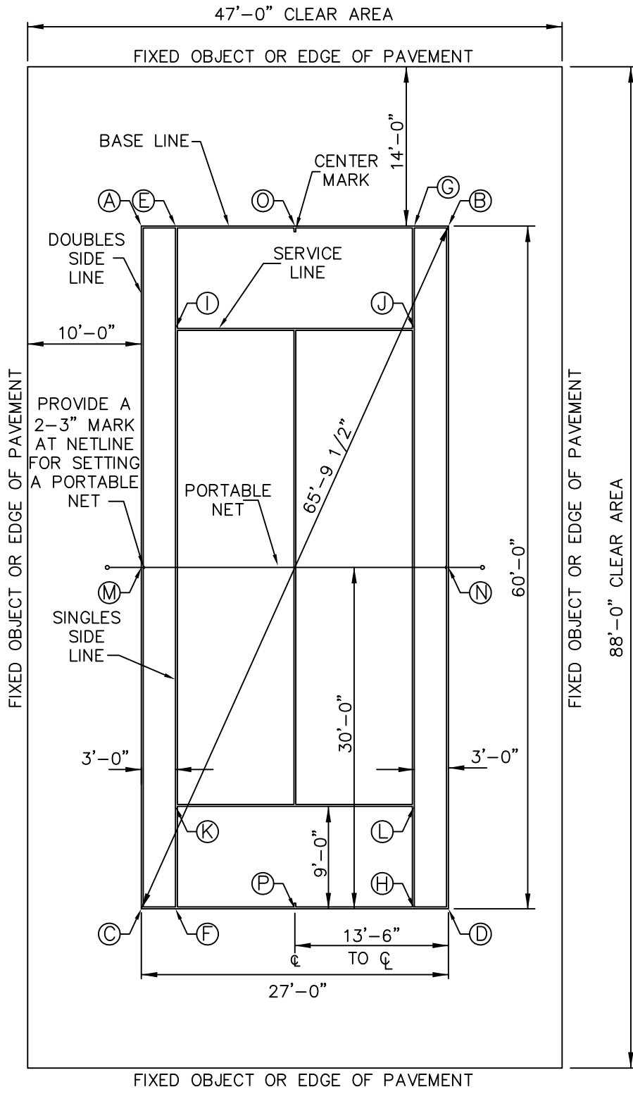
SINGLE COURT LINE LAYOUT NOT TO SCALE
